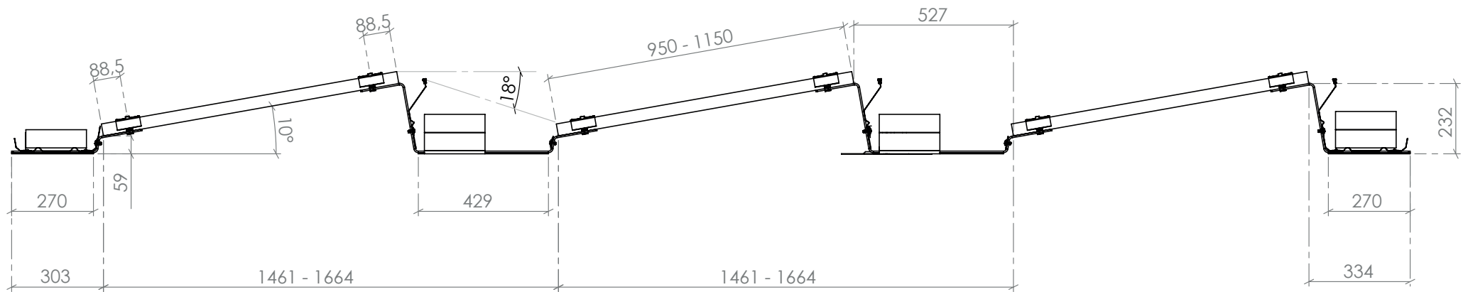
easyLIGHT S10 – 527 mm
