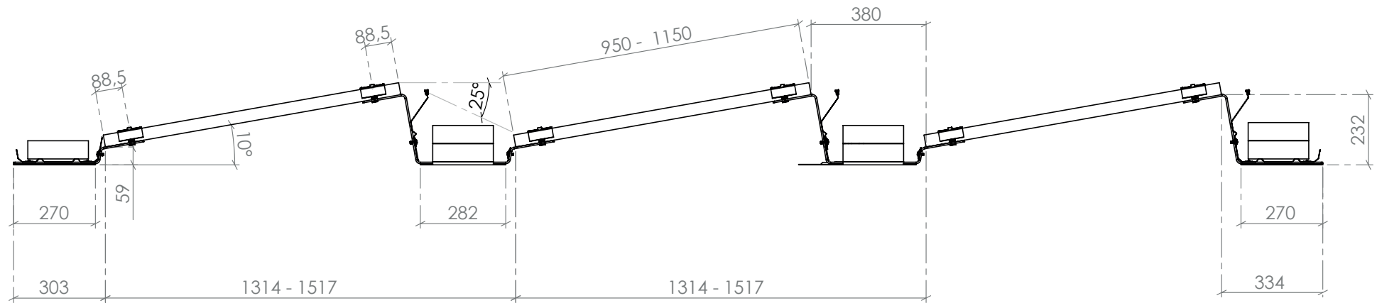
easyLIGHT S10 – 380 mm
